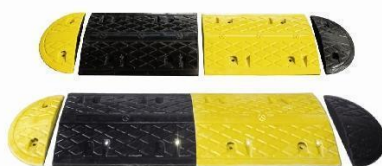
Model (型号): CC-B02 Centre Section (尺寸): 500x350x50mm, 500x350x45mm End Section (端头): 175x350x50mm
