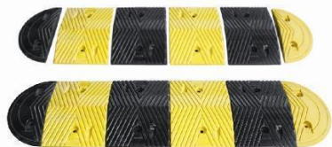
Model (型号): CC-B01 Centre Section (尺寸): 1000x350x50mm, 1000x350x42mm, 250x350x45mm End Section (端头): 175x350x45/50mm
